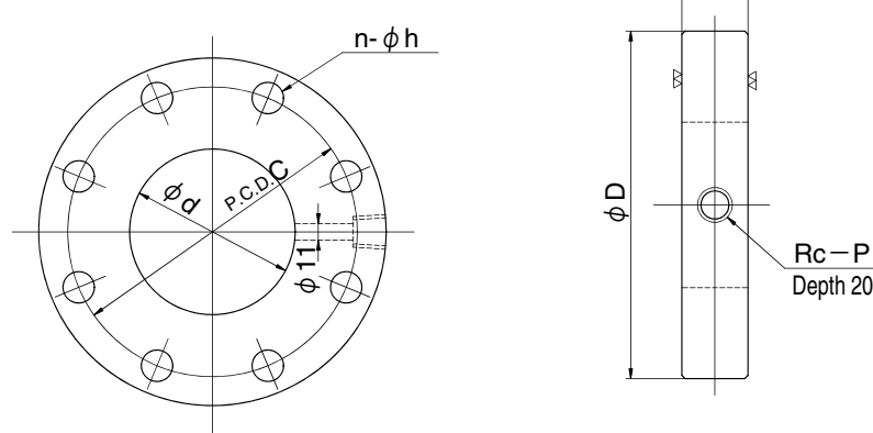
■ Dimensions Table (Unit: mm)
