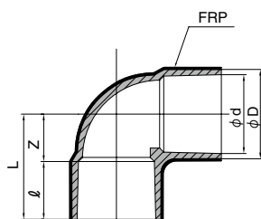
90° Elbow
