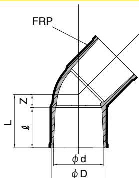
Elbow, Bend (45°)
