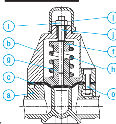
INSIDE STRUCTURE DIAGRAM
