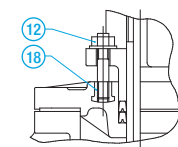
DETAILS OF SECTION "a"
