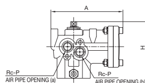
ACTUATOR SHAPE FOR PND-03S
